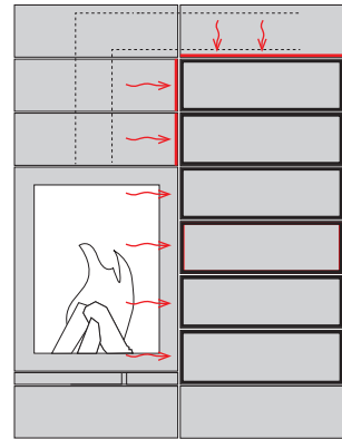
Technical box with radiation protection plate inserted
