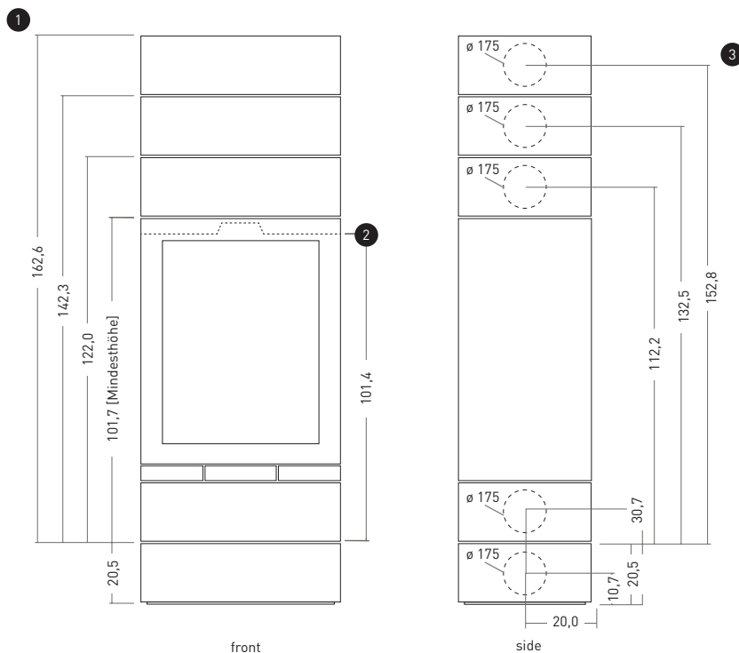
Smoke discharge (top)
