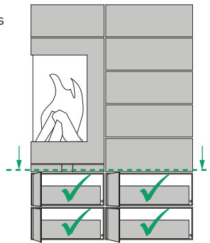
Correct installation:
